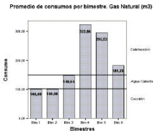
Fig.11: Consumos Gas Natural (m3)
